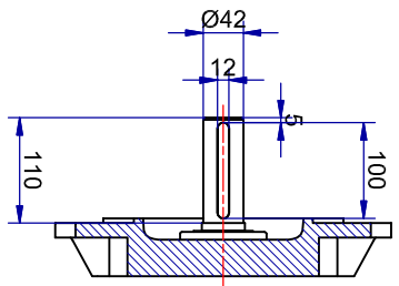
Shaft detail
