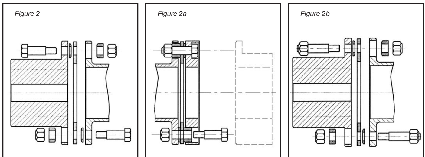
Figure 2 = Disc pack assembling diagram
