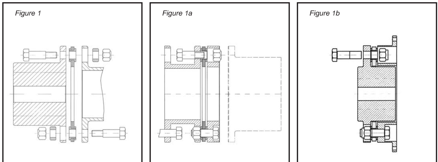
Figure 1 = Disc pack assembling diagram
