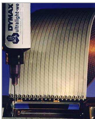
Lens Positioning
