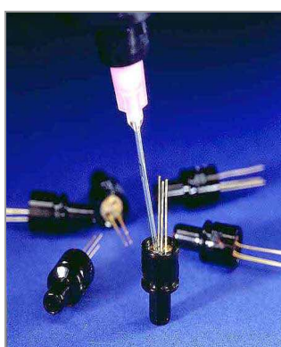
VCSEL Potting
