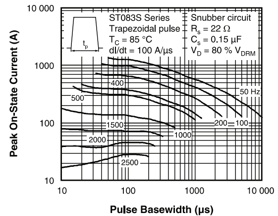
Fig. 13 - Frequency Characteristics
