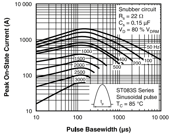
Fig. 11 - Frequency Characteristics
