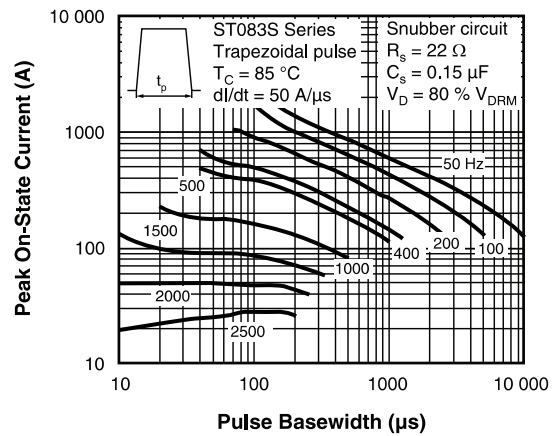
Fig. 12 - Frequency Characteristics
