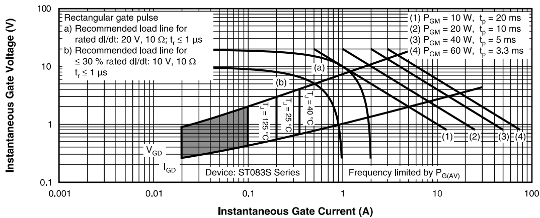
Fig. 15 - Gate Characteristics
