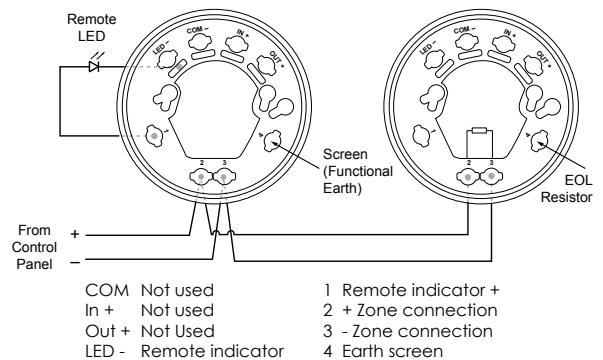
Sav-Wire base wiring connections
