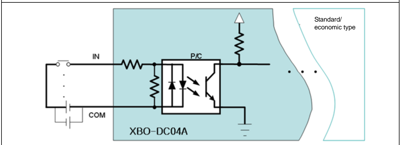
Circuit configuration
