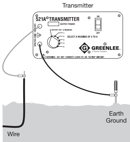
Figure 1 – Transmitter Setup
