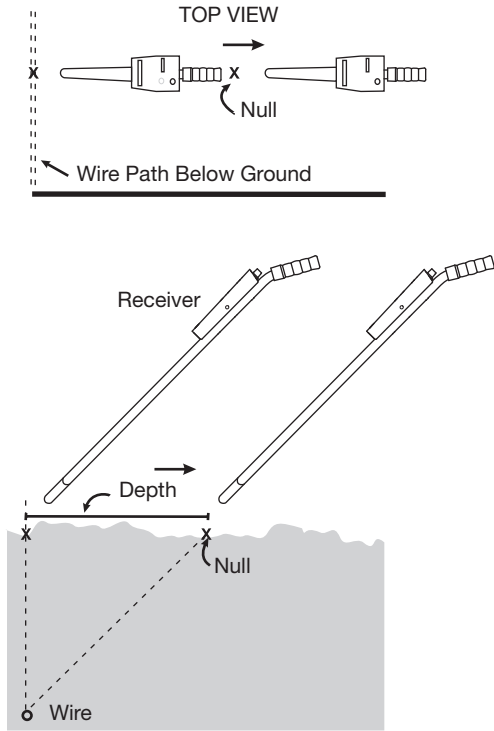
Figure 5 – Determining Depth
