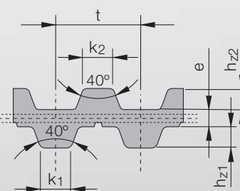
SYNCHROFLEX® Timing Belt (SFX) V-DL
